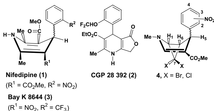
Figure 1. Structures of Nifedipine (1), CGP 28 392 (2), Bay K 8644 (3), and Methyl 7,7-dihalo-2-methyl-5-(nitrophenyl)-2-azabicyclo[4.1.0]hept-3-ene-4-carboxylates (4).
