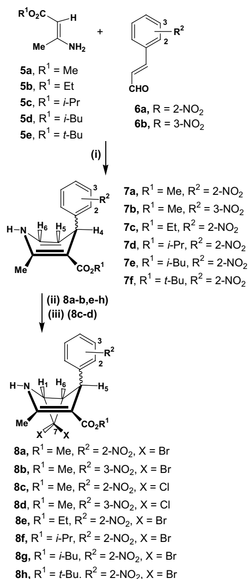
Scheme 1. Reagents and conditions: (i) piperidine, MeOH, reflux, 3 h (7a) and piperidine, EtOH, reflux, 6 h (7b–f); (ii) \text{PhHgCBr}_3 , dry benzene, reflux, 8 h; (iii) \text{PhHgCBrCl}_2 , dry benzene, reflux, 8 h.
